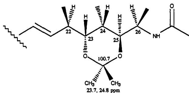
Coupling constants observed experimentally and calculated by molecular mechanics for acetonide methyl ester 4
