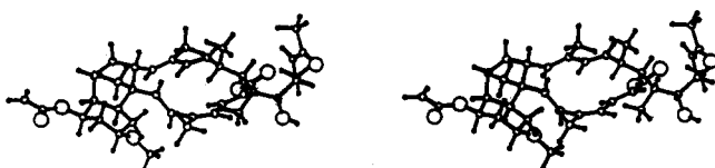
Figure 4. Stereoview of the lowest energy conformation of superstolide A (1).
