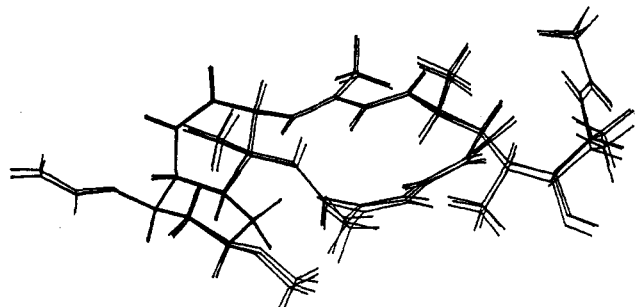
Figure 3. Three most stable conformations of 1 obtained from restrained molecular mechanics and dynamics calculations.
