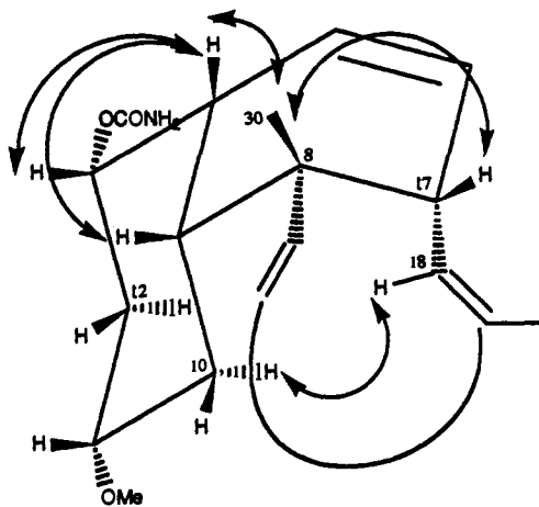
Chart 1. NOE Cross Peaks Observed in a 400-ms NOESY Spectrum (CDCl 3 ) of 1.
